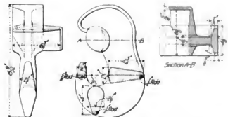
Figs. 4582-4584. Goodmann Wrecking Hook. Latrobe Steel & Coupler Co.
